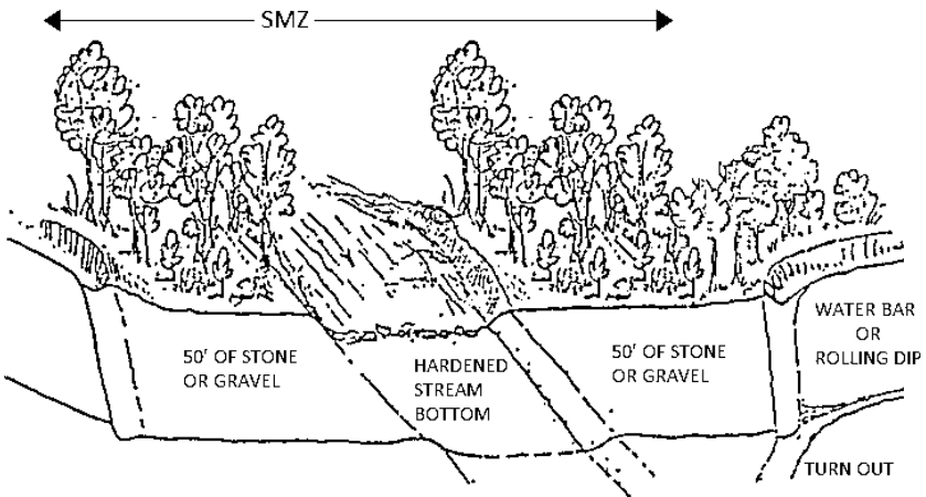
Low-water Crossing
